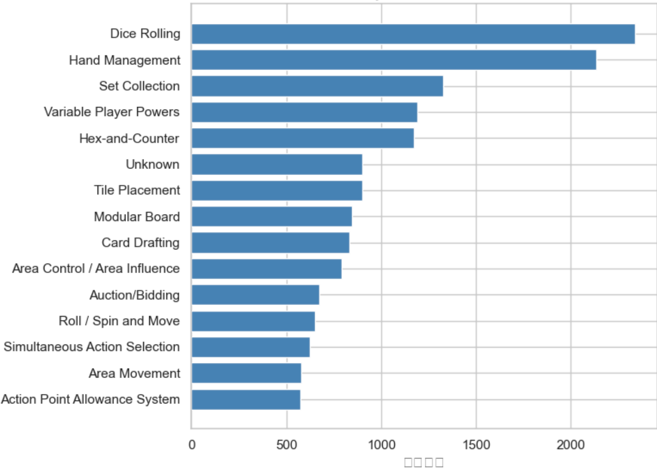
Top-15
